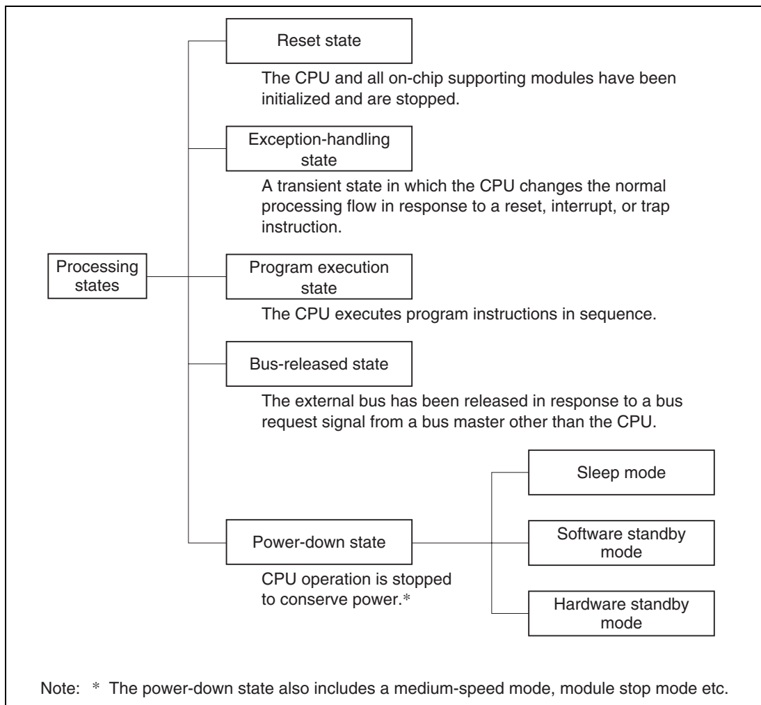
Figure 2.14 Processing States
