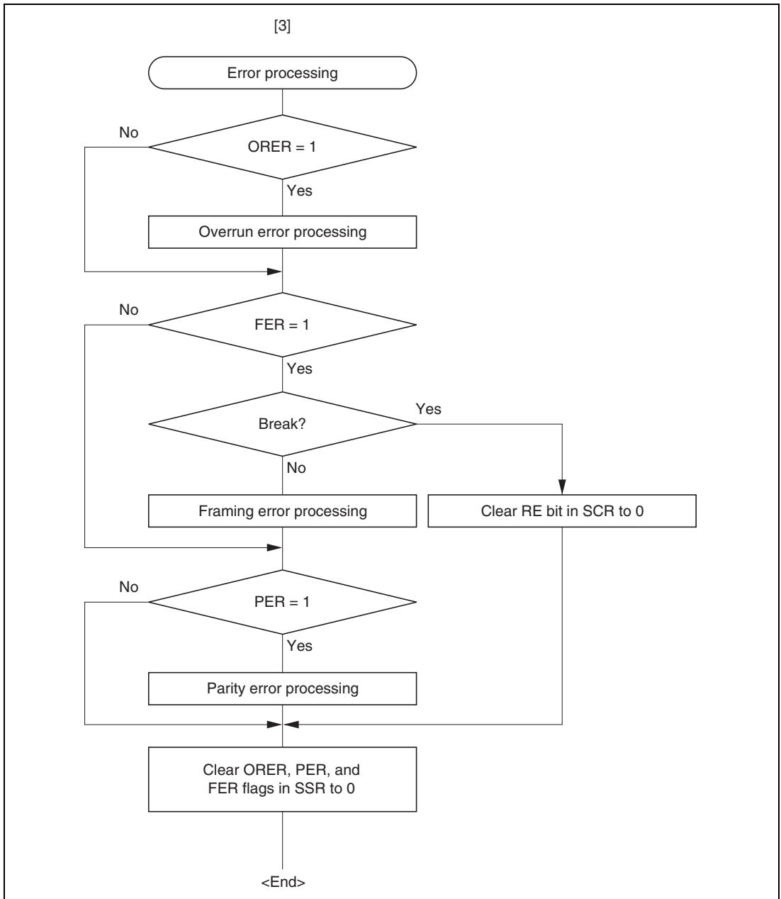
Figure 12.7 Sample Serial Reception Data Flowchart (cont)
