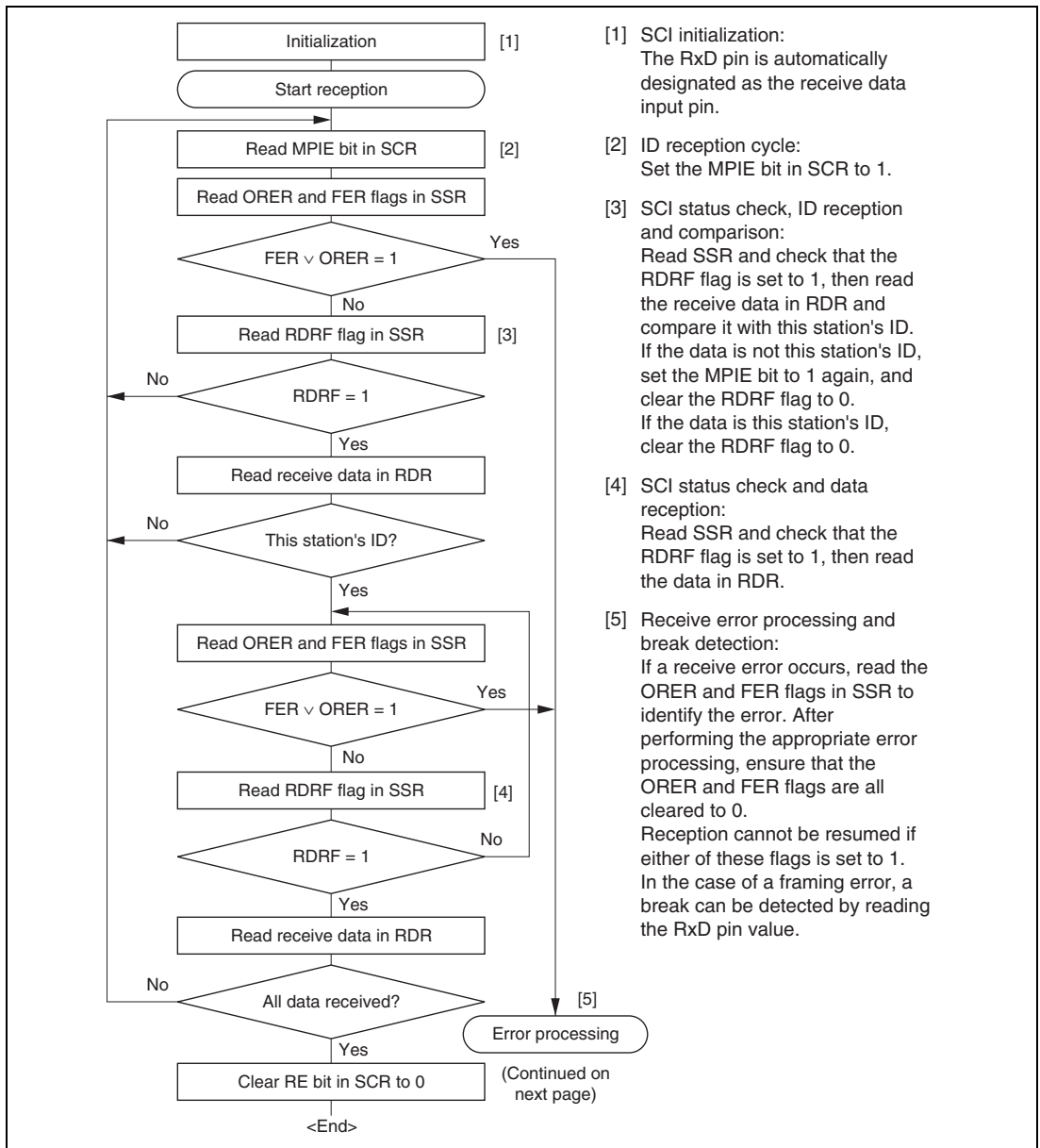
Figure 12.12 Sample Multiprocessor Serial Reception Flowchart
