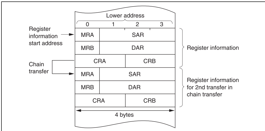
Figure 7.5 Location of Register Information in Address Space
