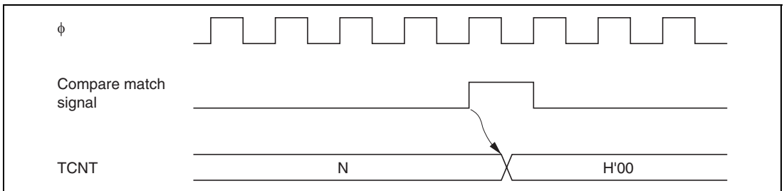
Figure 10.6 Timing of Compare Match Clear
