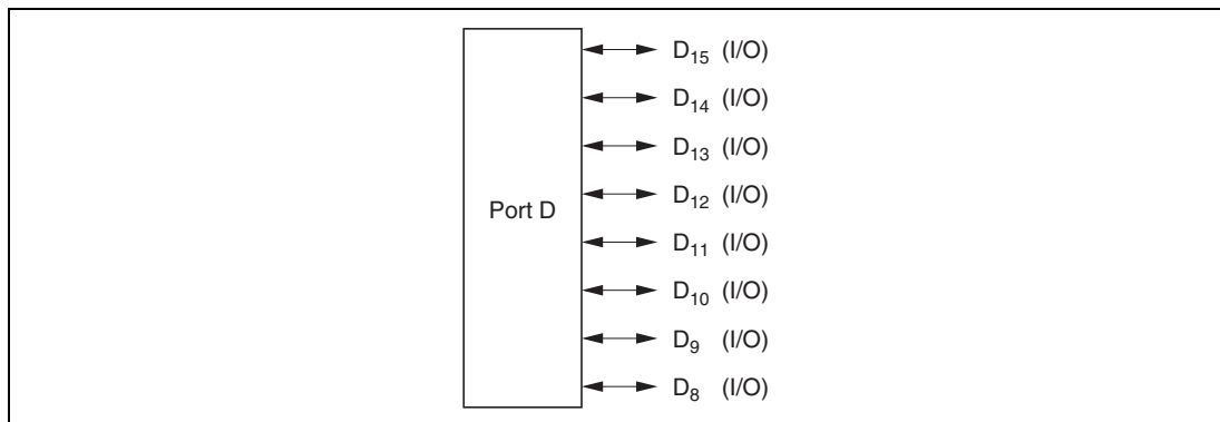
Figure 8.20 Port D Pin Functions (Modes 1, 2, 4, 5, and 6)
